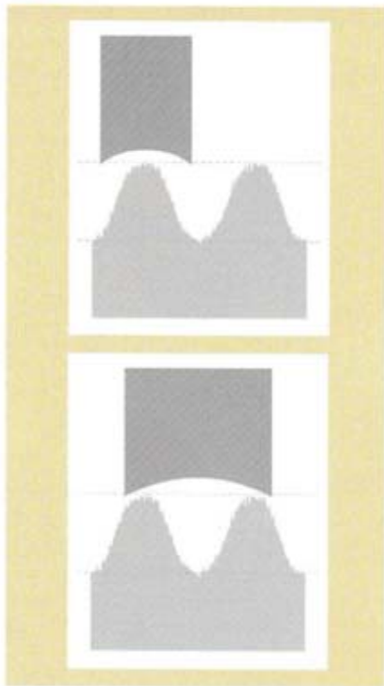
Fig. 1—While superfinishing can put a mirror finish on the part, it may also be used to improve roundness, depending on the incoming roundness of the workpieces and the width of the stones. Narrow stones (above) ride up and down on the lobes to improve surface finish only. Wider stones (below) can bridge the lobes to reduce their depth (that is, to improve roundness) and impart a high degree of surface finish at the same time.
