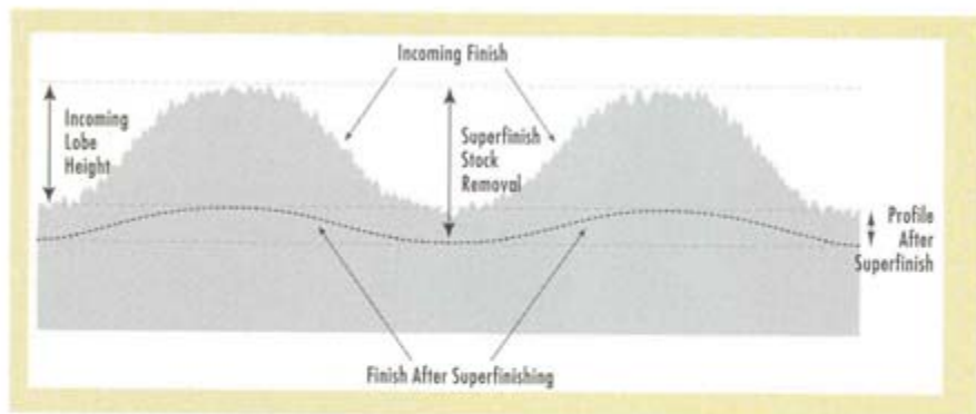
Fig. 2—Superfinishing can improve roundness in cases of moderate lobing.
