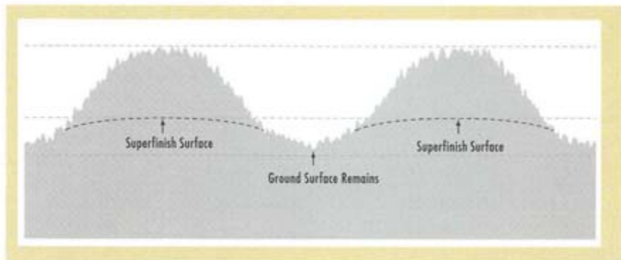
Fig. 3—Excessive lobing cannot be totally corrected with superfinishing. In fact, superfinishing may create unacceptable chatter lines, causing the piece to be rejected.
